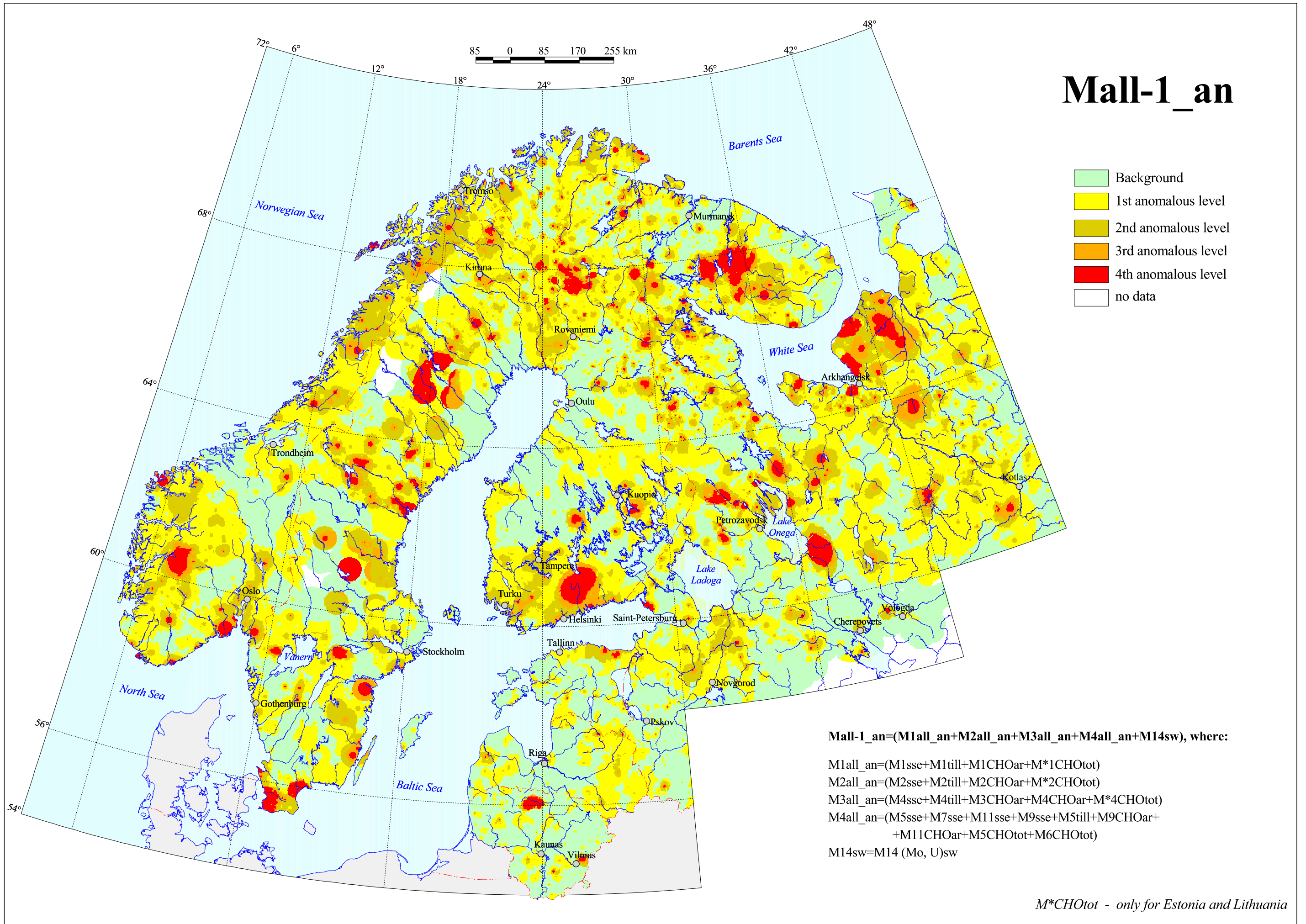
Integrated Anomalous Geochemical Fields, Mall-1_an
